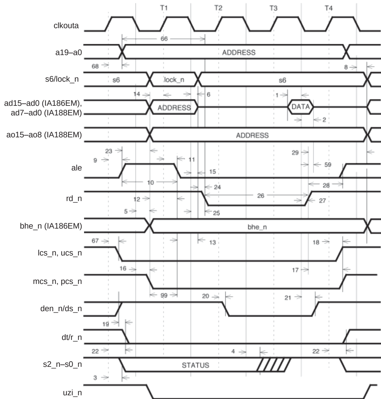
Figure 11. Read Cycle
